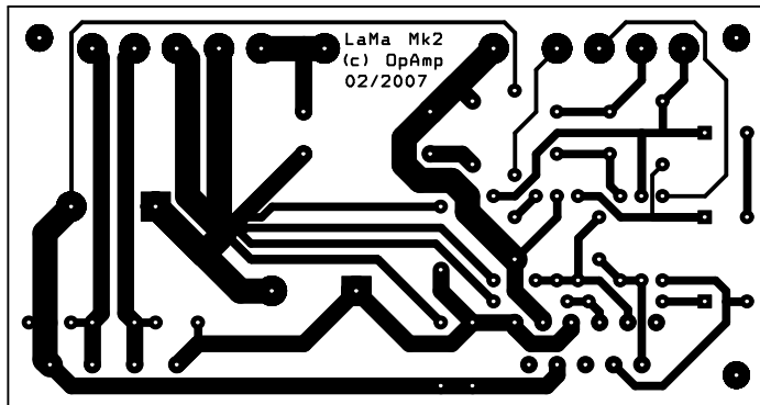
LaMa Mk2 copper side
